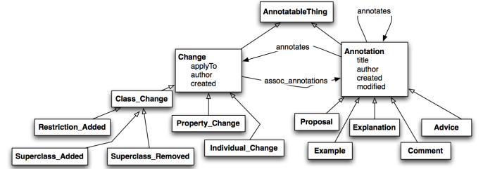
Figure 2: Excerpt of the Change and Annotation Ontology (ChAO) used by Protégé [23]. Boxes represent classes and lines represent relationships.
