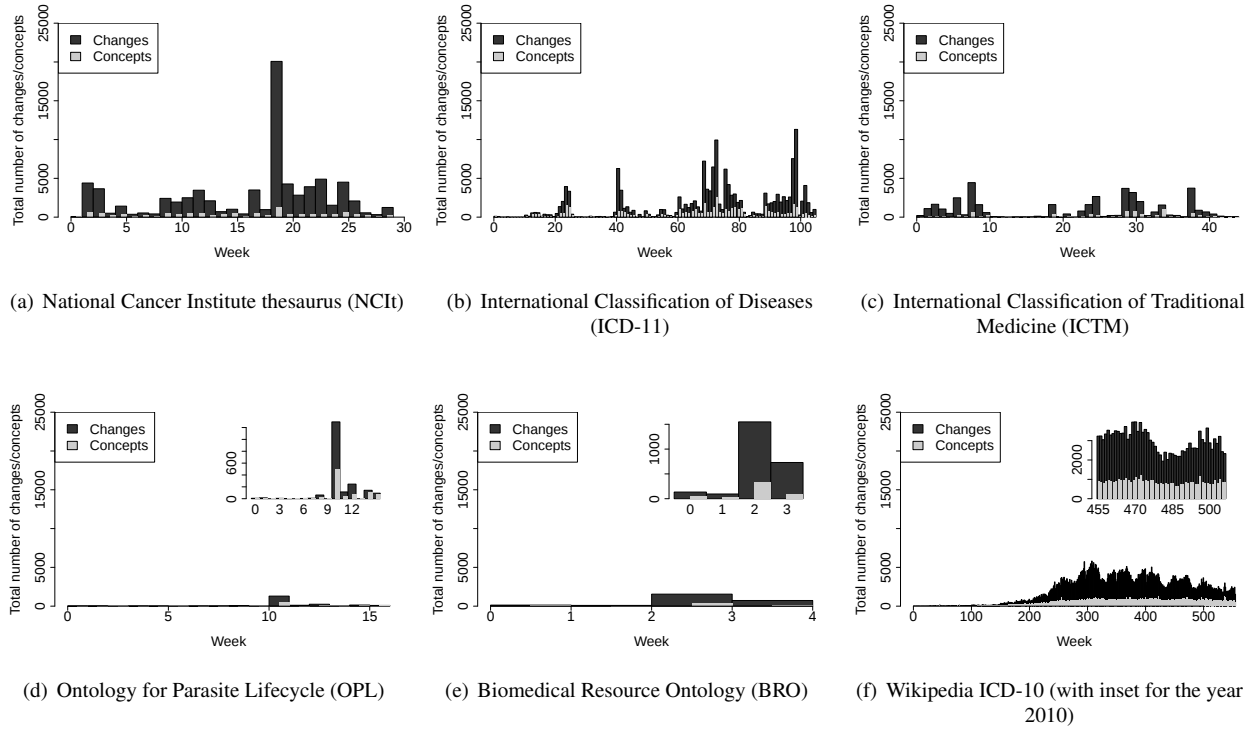
Figure 4: Weekly number of changes in our five collaborative ontology engineering projects NCIt, ICD-11, ICTM, OPL, BRO, and in Wikipedia ICD-10 (for comparison). Black bars represent changes, grey bars represent distinct concepts that have been changed. Note that the x-axis is scaled differently for each project due to differences in the change log durations. The inset for Wikipedia ICD-10 magnifies the number of changes and concepts for a period of 52 weeks (one year) to highlight seasonal fluctuations. The insets for OPL and BRO are of smaller scale on the y-axis for reasons of readability.
