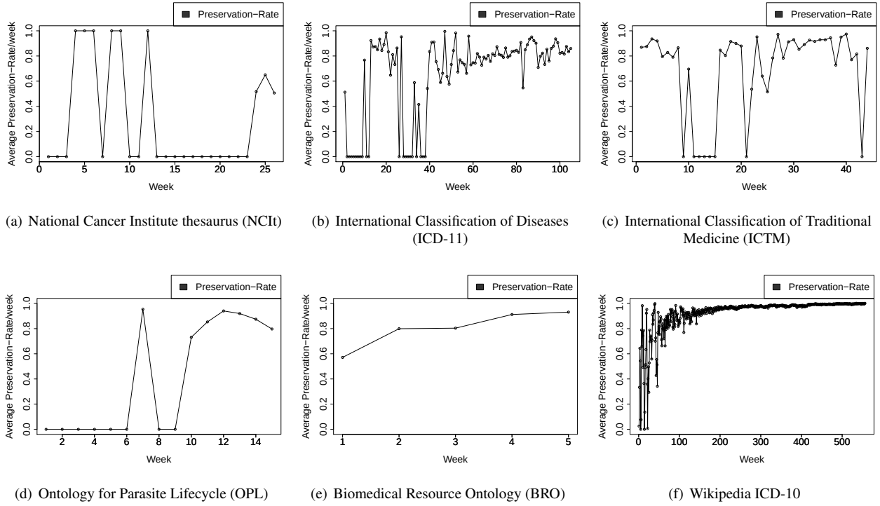
Figure 11: Average preservation rate per change during week T (sliding window of 1 week) in our five collaborative ontology engineering projects NCIt, ICD-11, ICTM, OPL, BRO, and in Wikipedia ICD-10 (for comparison). The preservation rates of all changes which modify textual attributes and were performed during each week have been accumulated and then divided by the number of changes performed. The preservation rate ranges from 0 indicating that the texts of a concepts textual properties have been completely replace with newly entered text, to 1, indicating that the texts of a concepts properties have not been changed. Note that the x -axis is scaled differently for each project due to differences in the change log durations. Weeks that show an average preservation rate of 0 are weeks where no modifying changes have been performed.
